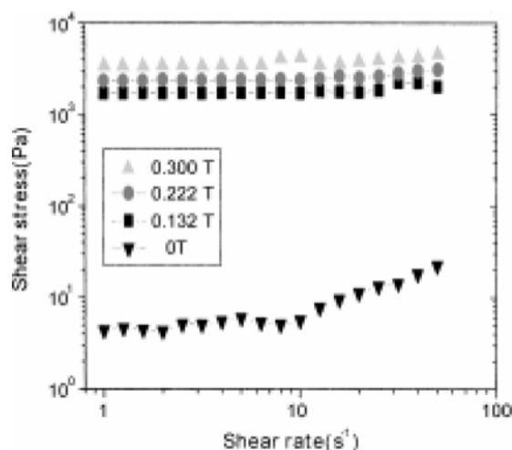
Fig. 7. Steady shear stress versus shear rate for carbonyl iron dispersed in viscoelastic medium (grease 25 w%, \text{CrO}_2 10 w%).
